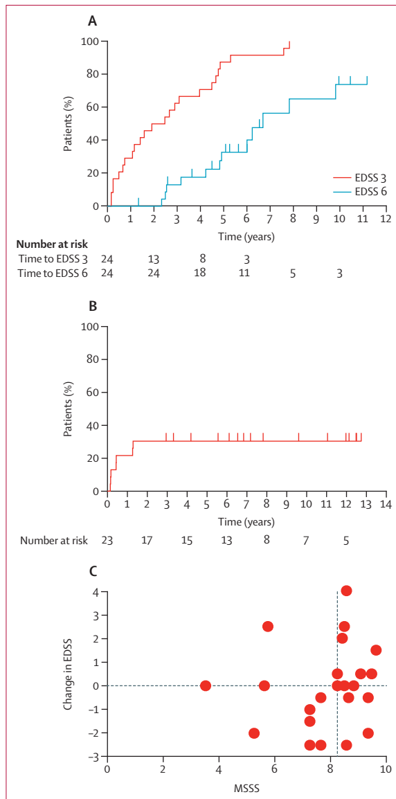
Figure 3: Progression of disabilities before and after autologous haemopoietic stem-cell transplantation (A) Time from diagnosis to a sustained EDSS of 3.0 and EDSS of 6.0. Patients reached EDSS 3.0 after a median of 2.2 years, and EDSS 6.0 after a median of 6.7 years from diagnosis. (B) Time from autologous haemopoietic stem-cell transplantation to sustained accumulation of additional disability. (C) Relation between the MSSS and change in the EDSS between the latest follow-up assessment and the final assessment before autologous haemopoietic stem-cell transplantation, showing that disability is more likely to improve for patients with an MSSS less than or equal to 8.3 just before autologous haemopoietic stem-cell transplantation; positive predictive value 90.9% (95% CI 58.7–99.8). EDSS=Expanded Disability Status Scale. MSSS=Multiple Sclerosis Severity Score.
